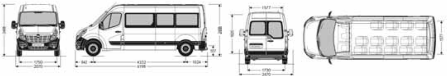
Bus L3H2
