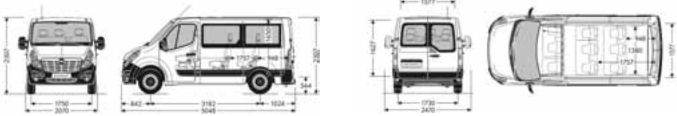
Combi L1H1
